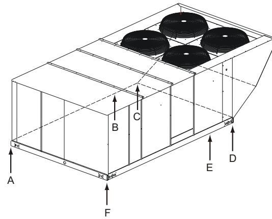
ZT unit 6 point load weight
